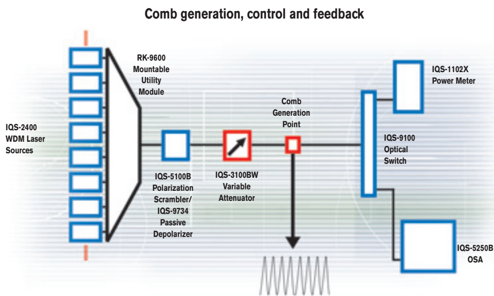
Typical setup for an IQS-based optical fiber amplifier test system using the IQS-2400 WDM Laser Source.
