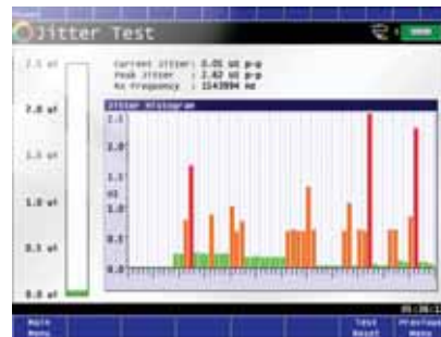
Example Jitter Measurement Screen
