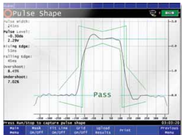
Example Pulse Mask Measurement Screen
