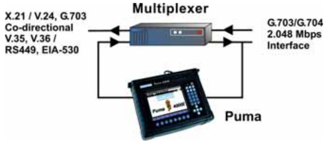
2 Mbps Multiplex Analysis
