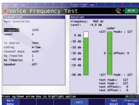
Example Voice Frequency Analysis Screen
