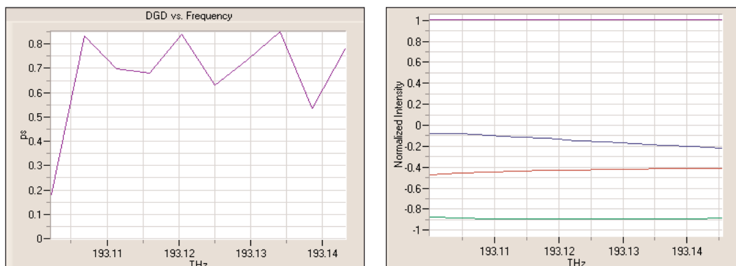
Figure 14. DGD (a) and Stokes vectors (b) of the 25-GHz fiber Bragg grating.
