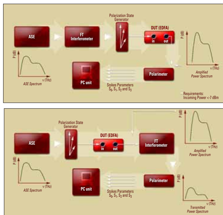
Figure 18 (a). The FPMD-5600 allows testing EDFAs in low-gain regime (a) as well as in high-gain or saturation modes (b).
