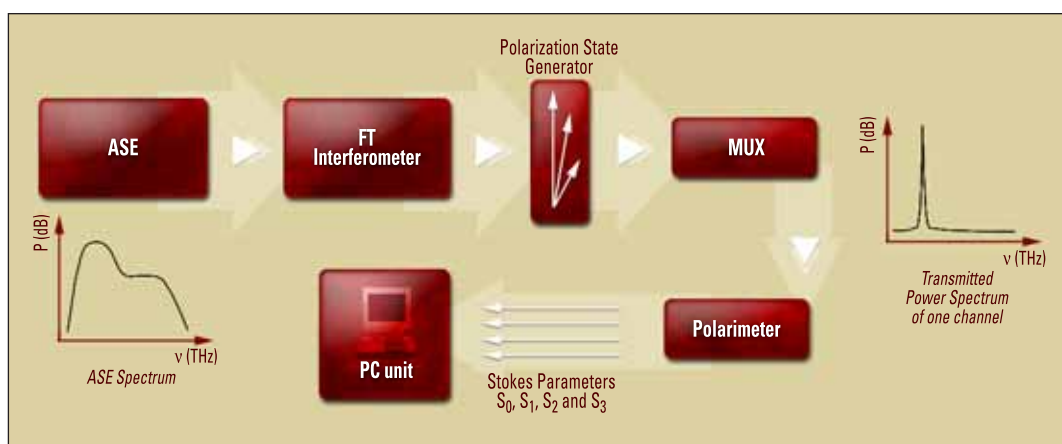
Figure 8. Connection scheme for a passive narrowband device (MUX) functioning in transmission.
