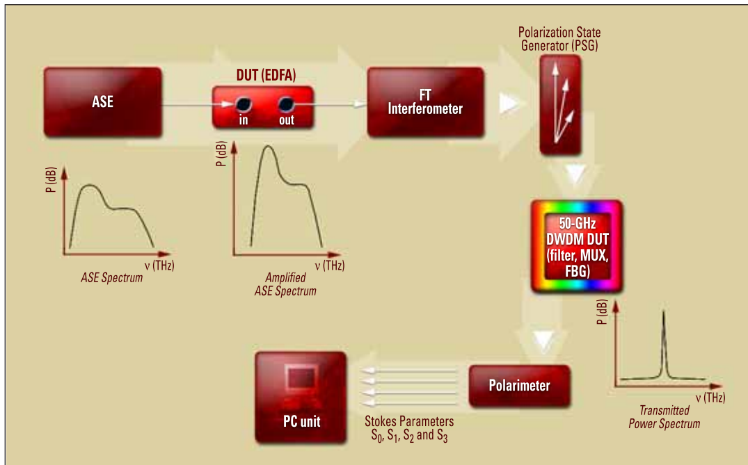
Figure 21. Schematic diagram of a PMD test setup incorporating both active and passive devices.
