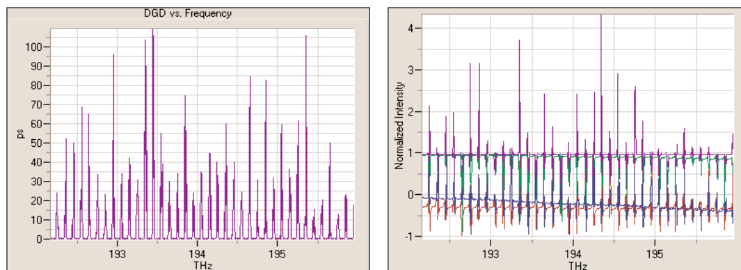
Figure 16. DGD curve (a) and Stokes traces (b) of the interleaver. Clear windows (transmission windows) show very low PMD values.
